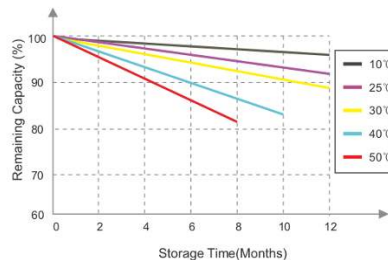
SELFDISCHARGE CHARACTERISTICS
