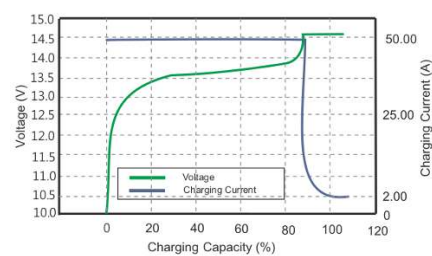
CHARGING CHARACTERISTICS
