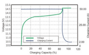
CHARGING CHARACTERISTICS
