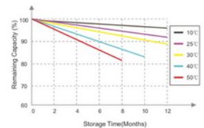
SELF-DISCHARGE CHARACTERISTICS
