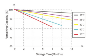
SELF-DISCHARGE CHARACTERISTICS
